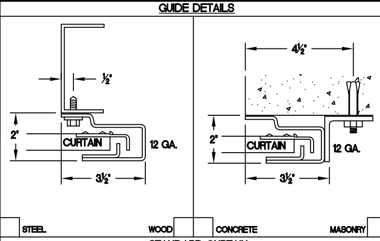
STANDARD CURTAIN
