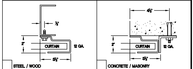
GUIDE DETAIL (NON-WINDLOCK)
