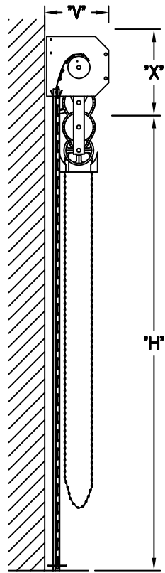
SECTION-A-A
